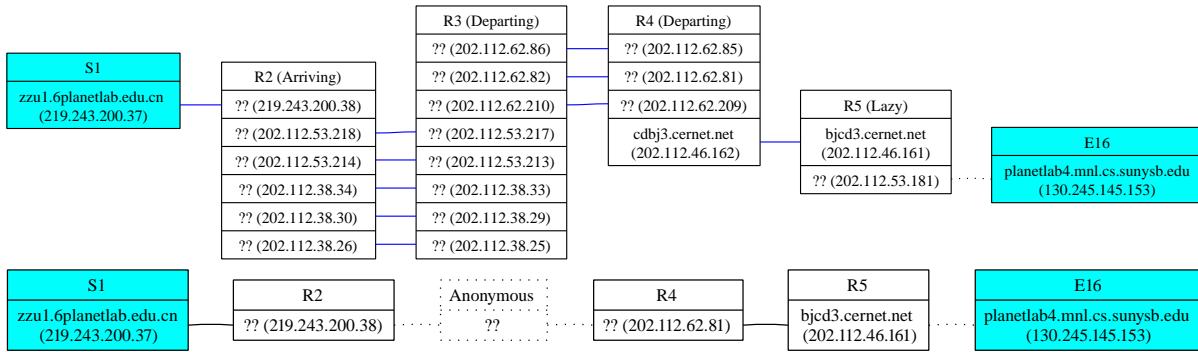
Figure 2: Partial Trace from Zhengzhou University, China to SUNY Stony Brook, USA; inferred by DisCarte (top) and Rocket-fuel techniques (bottom). DisCarte finds many load-balanced paths through an anonymous router (R3) and helps determine the implementation class of each device along the path.
